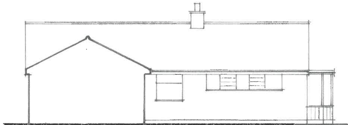
SIDE ELEVATION. 1-100
