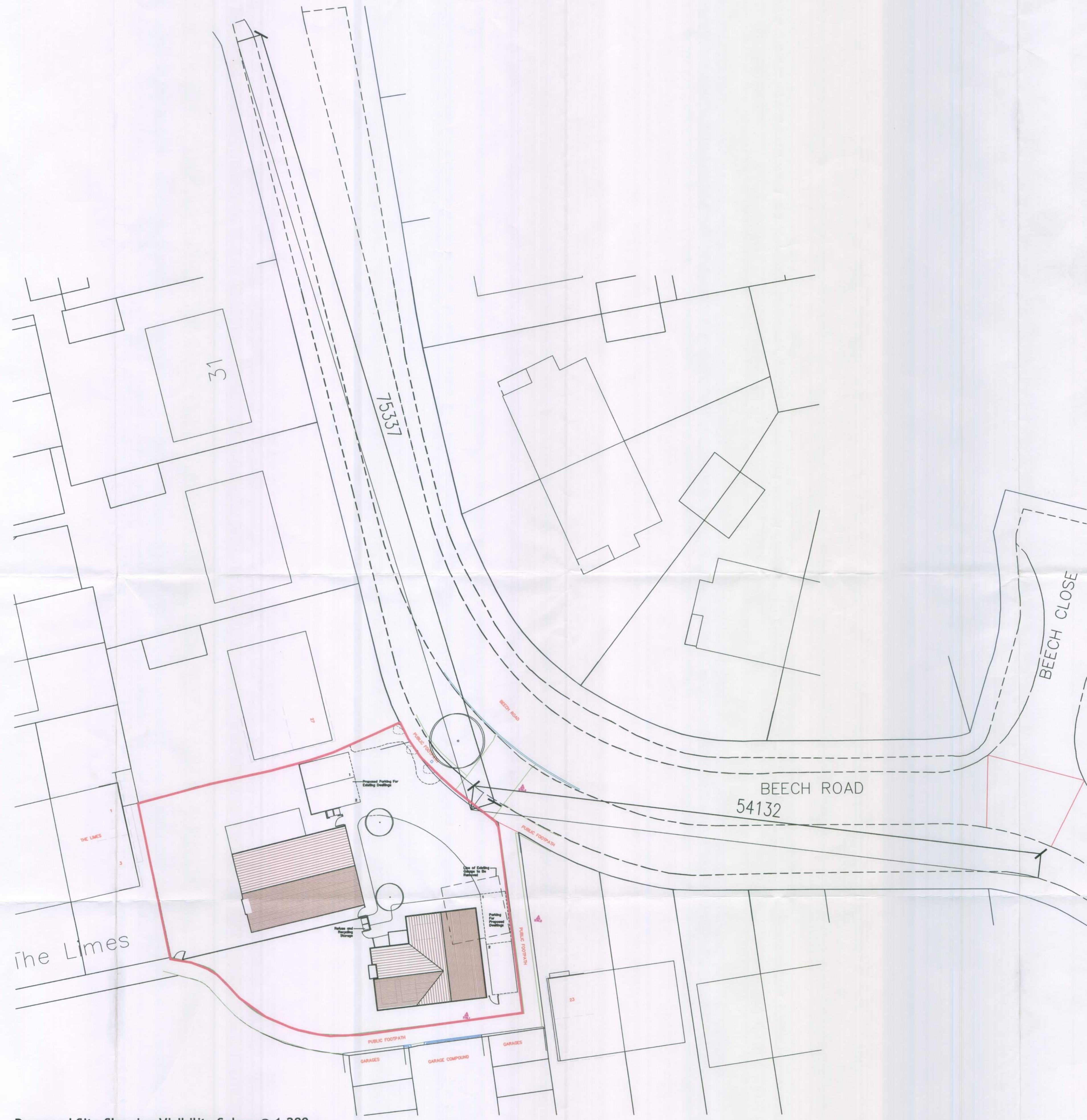
Proposed Site Showing Visibility Splays @ 1:200
