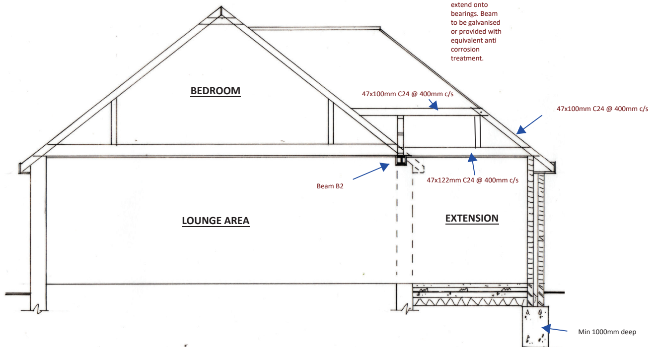
SECTION 1:50
