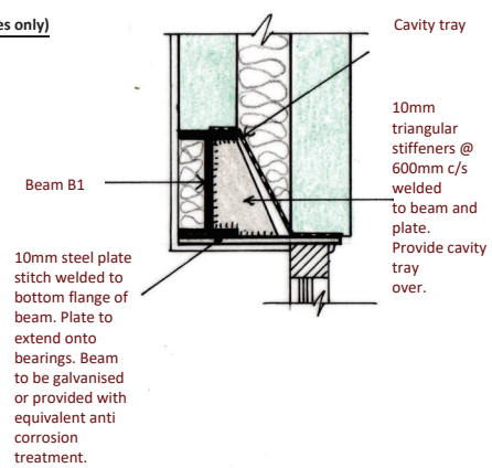
BEAM B1 DETAIL
