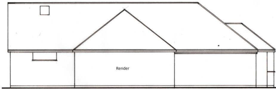
EXISTING SIDE ELEVATION (WEST) 1:100
