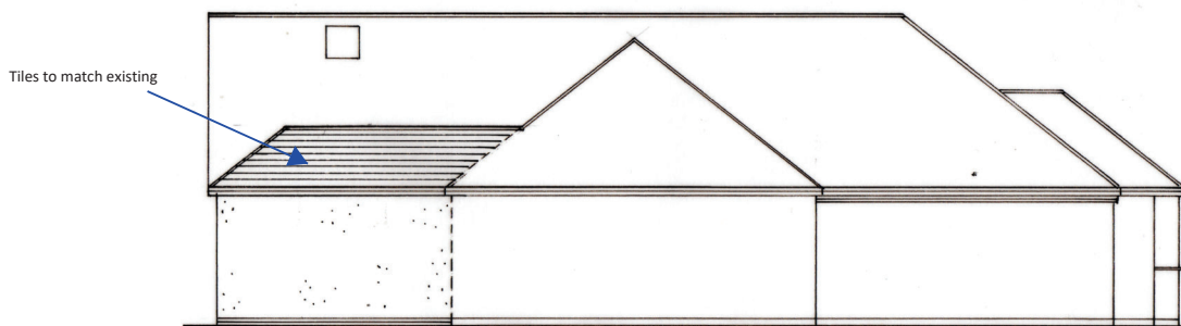
PROPOSED SIDE ELEVATION (WEST) 1:100
