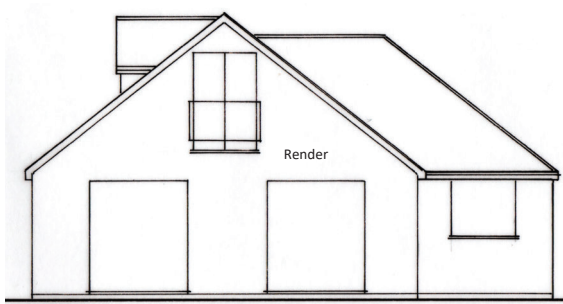
EXISTING REAR ELEVATION (NORTH) 1:100
