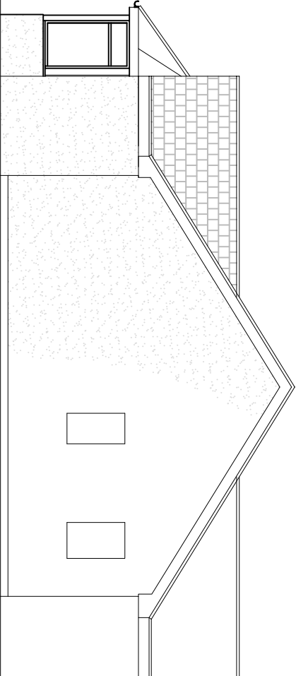
EAST ELEVATION
