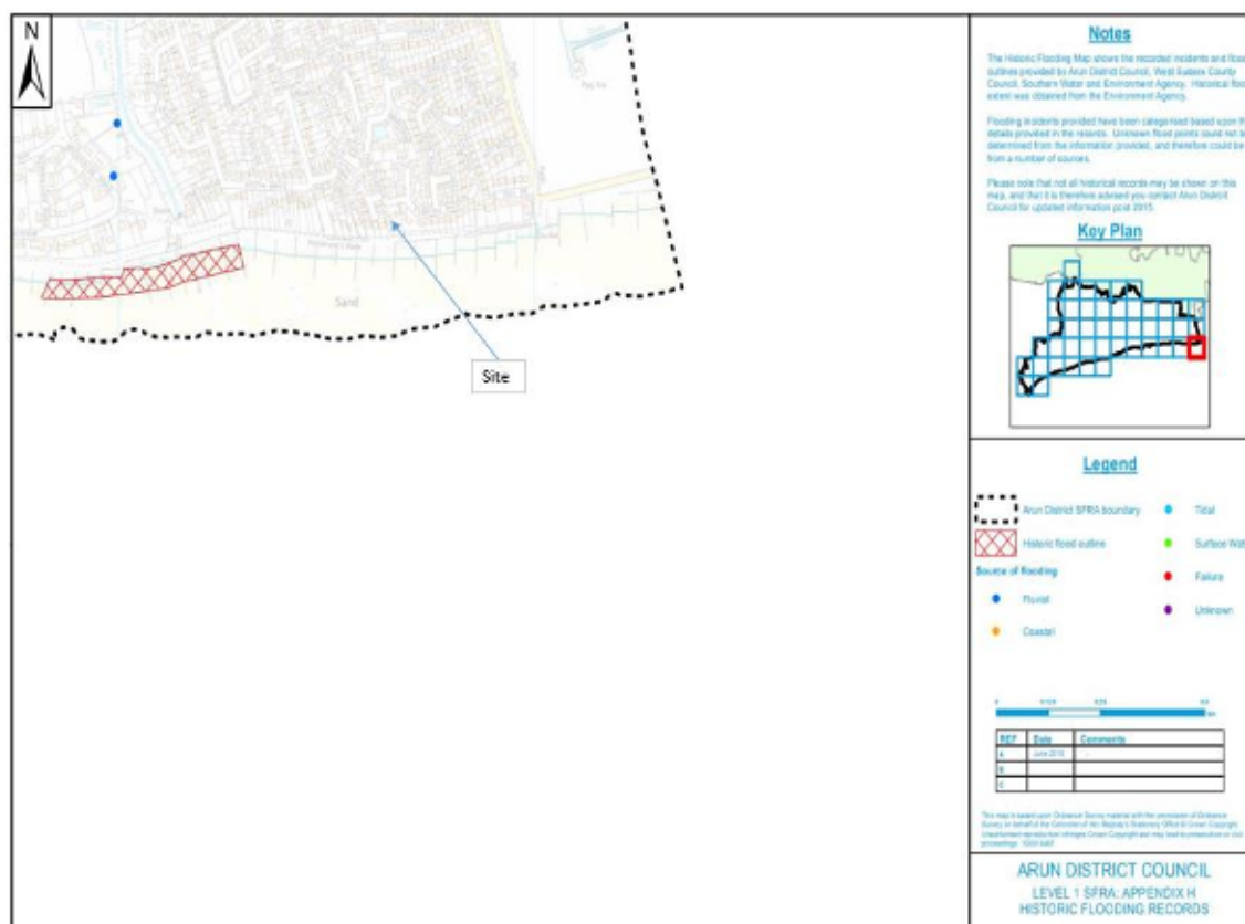
Figure 10 Historical Flooding. (Source: EA)
