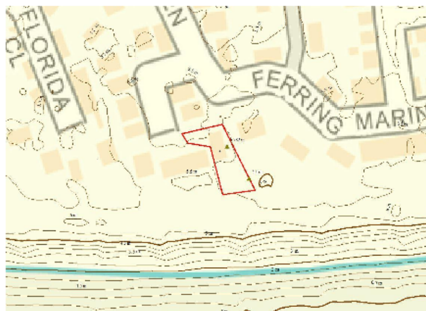
Figure 2 Topography (Source: Global Mapper and EA 2m LiDAR)
