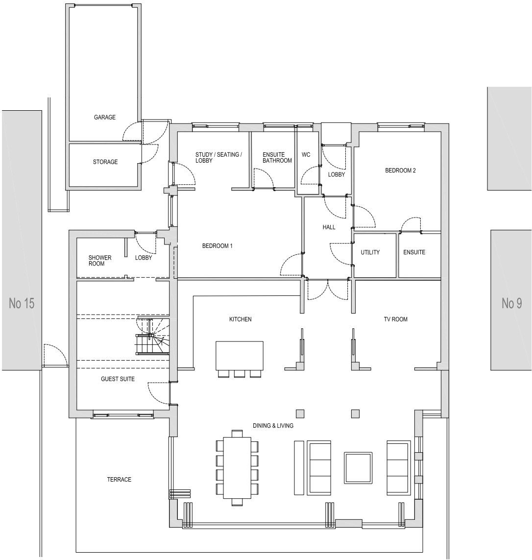
Existing ground floor at 1:100 @ A3
