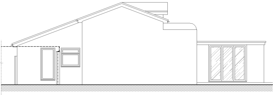
Existing West elevation at 1:100 @ A3
