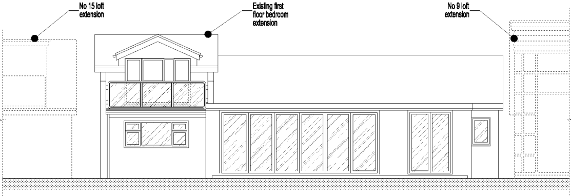
Existing South / garden elevation at 1:100 @ A3
