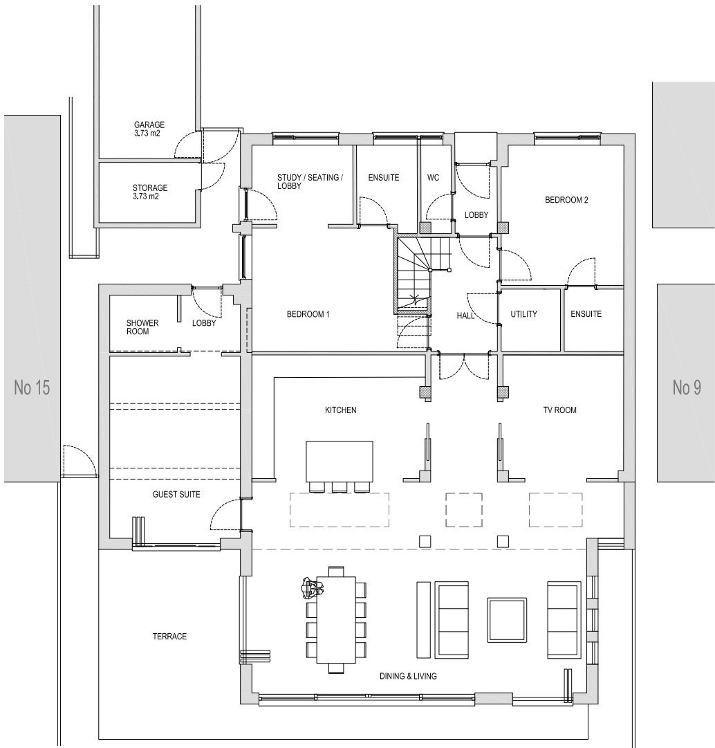
Proposed ground floor at 1:100 @ A3
