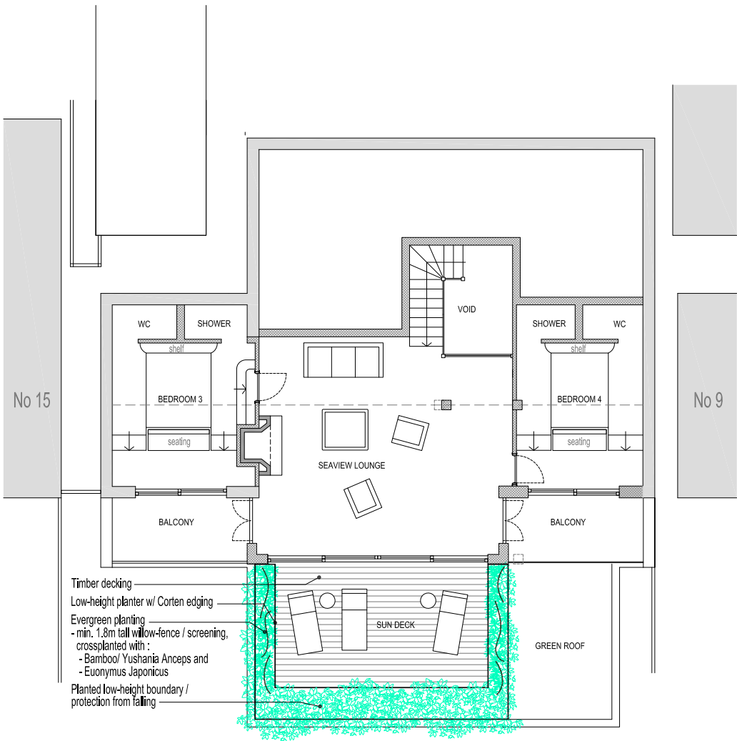
Proposed first floor at 1:100 @ A3
