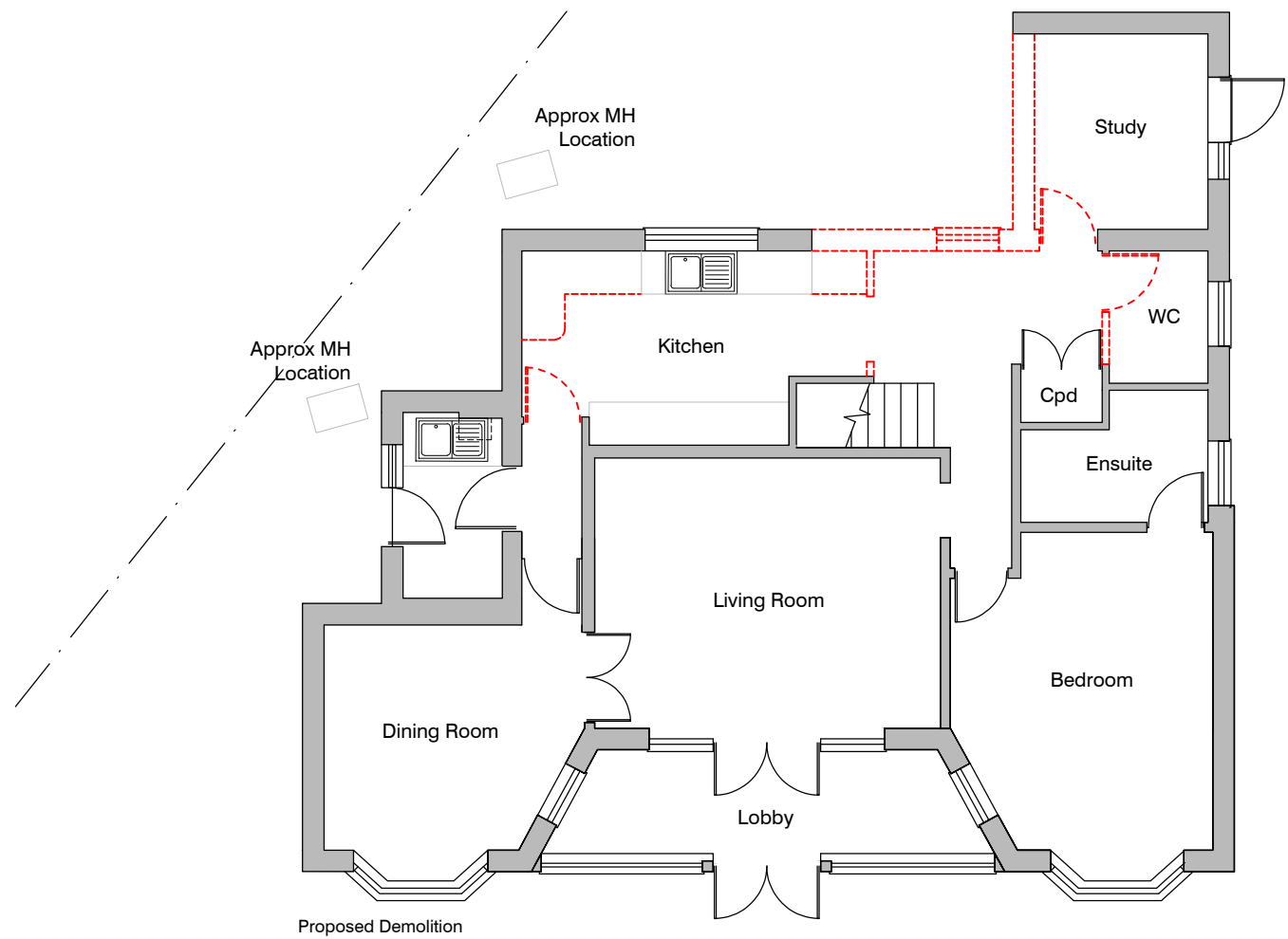
Proposed Demolition
