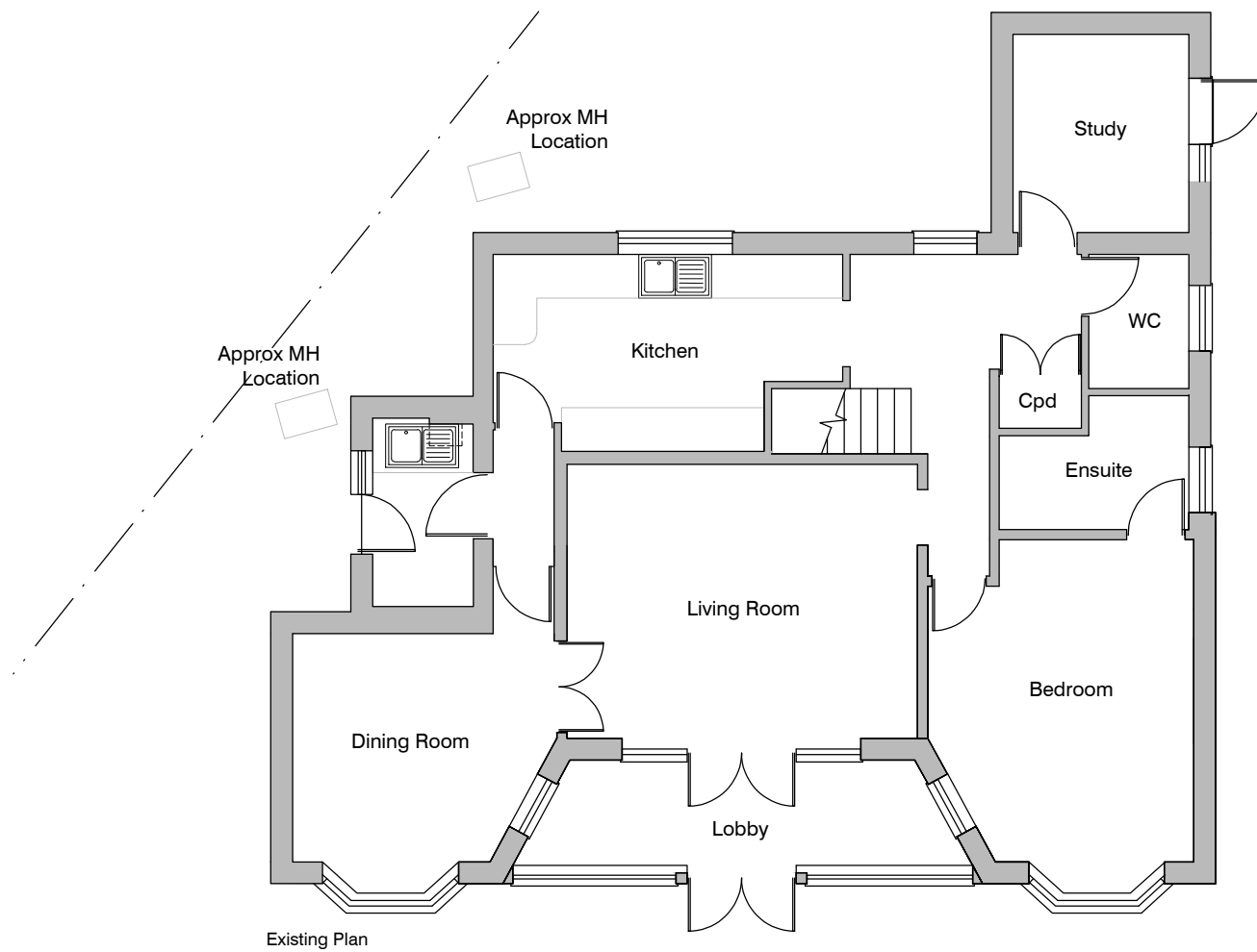
Existing Plan
