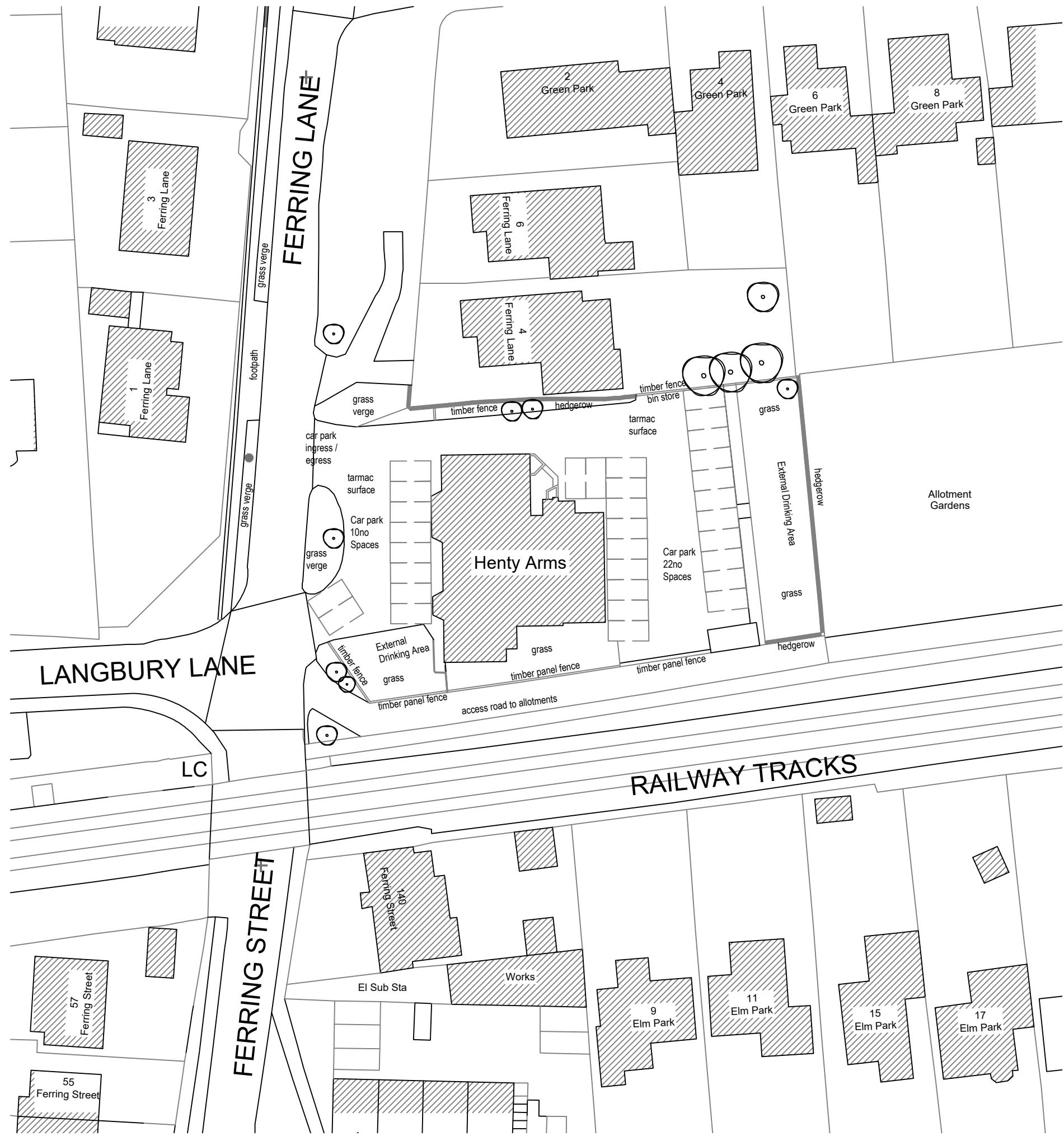
Existing Site Block Plan Scale 1/500
