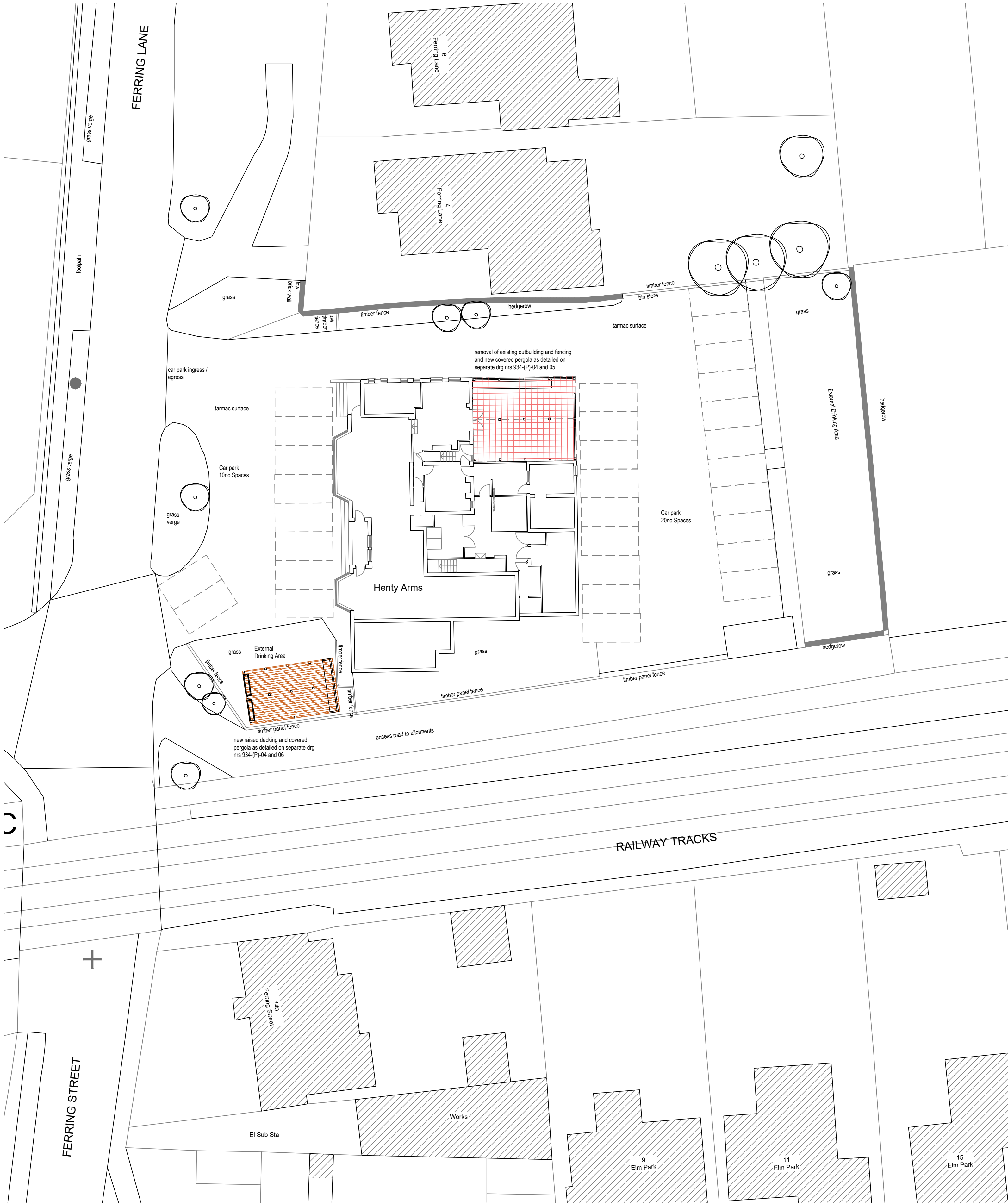
Proposed Layout Plan Scale 1/200
