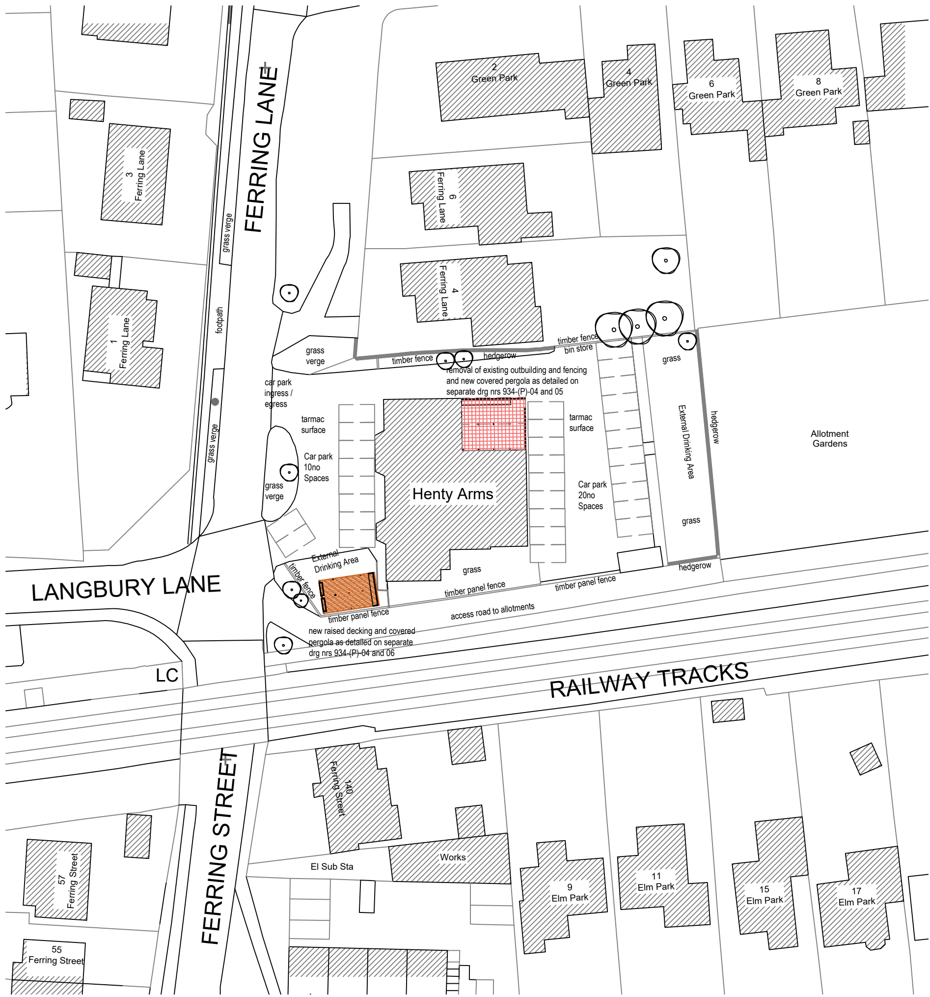
Proposed Site Block Plan Scale 1/500
