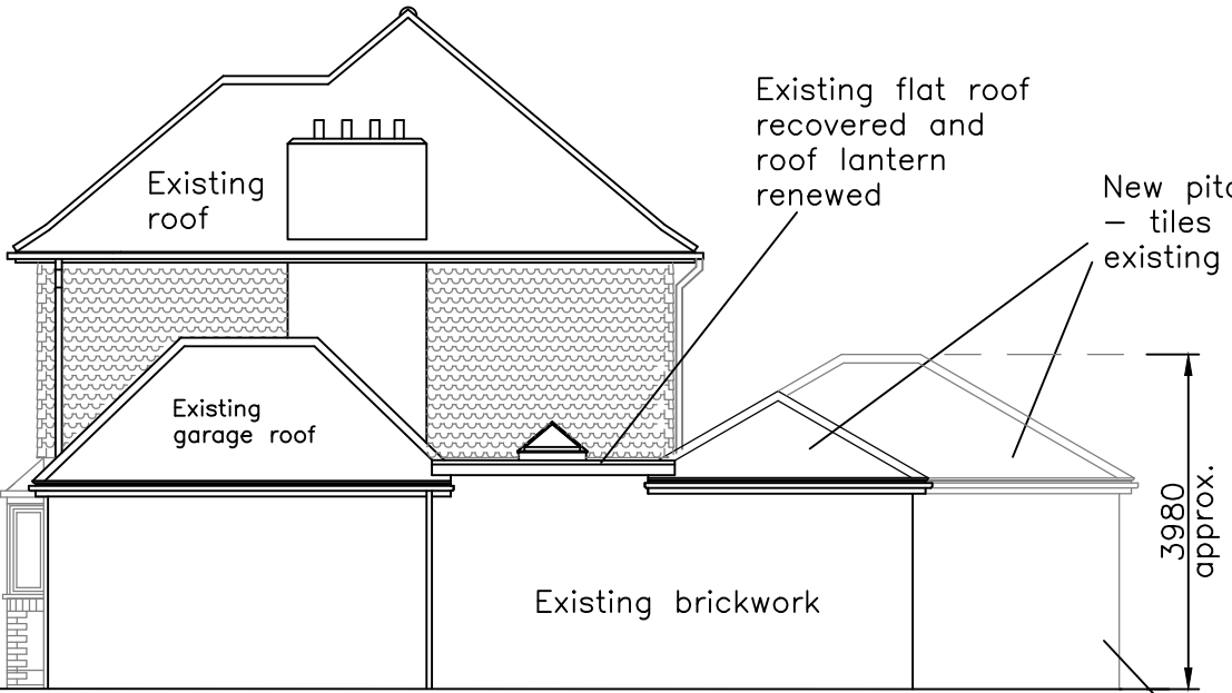
East Elevation
