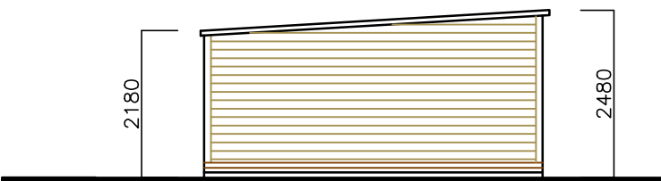
West Elevation 1:100
