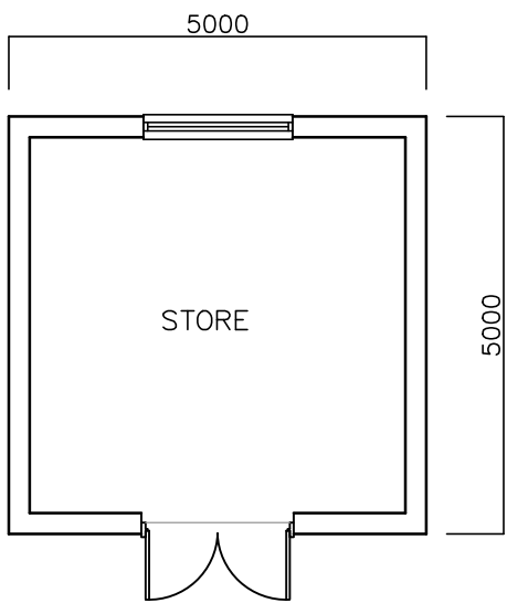
Floor Plan 1:100
