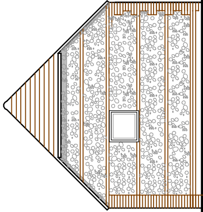
East Elevation 1:100
