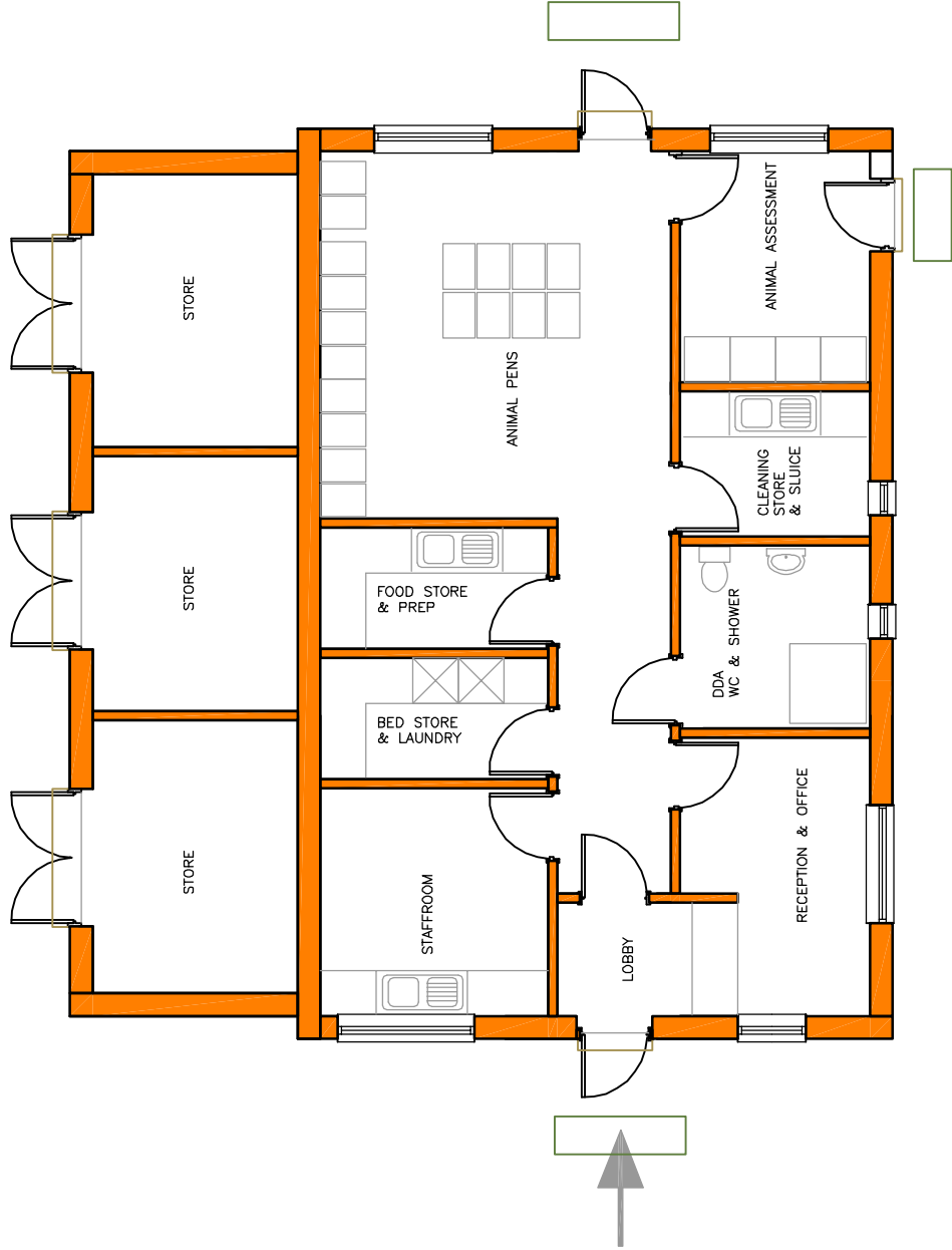
WILDLIFE REHABILITATION UNIT Floor Plan 1:100
