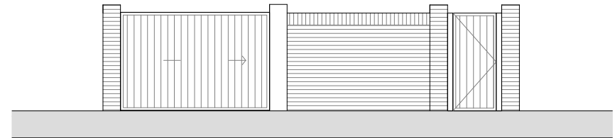
PROPOSED elevation looking south from driveway
