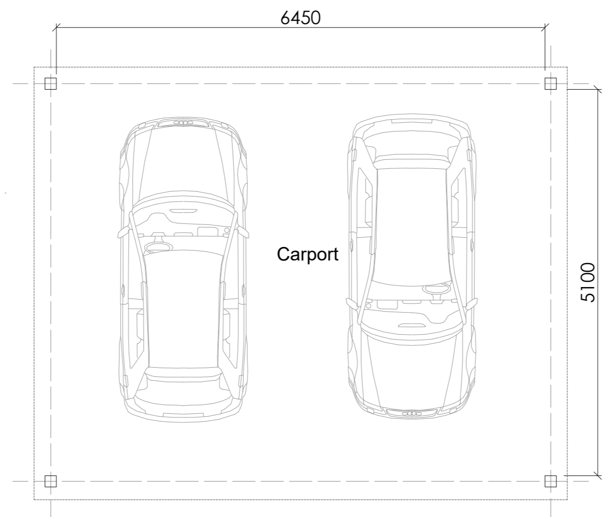
PROPOSED CARPORT PLAN
