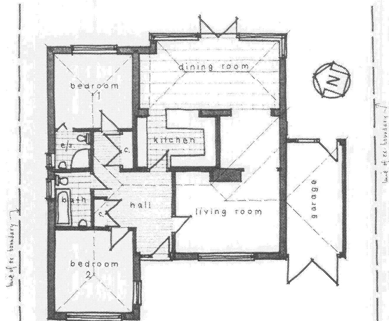
GROUND FLOOR PLAN 1:100 @ A3
