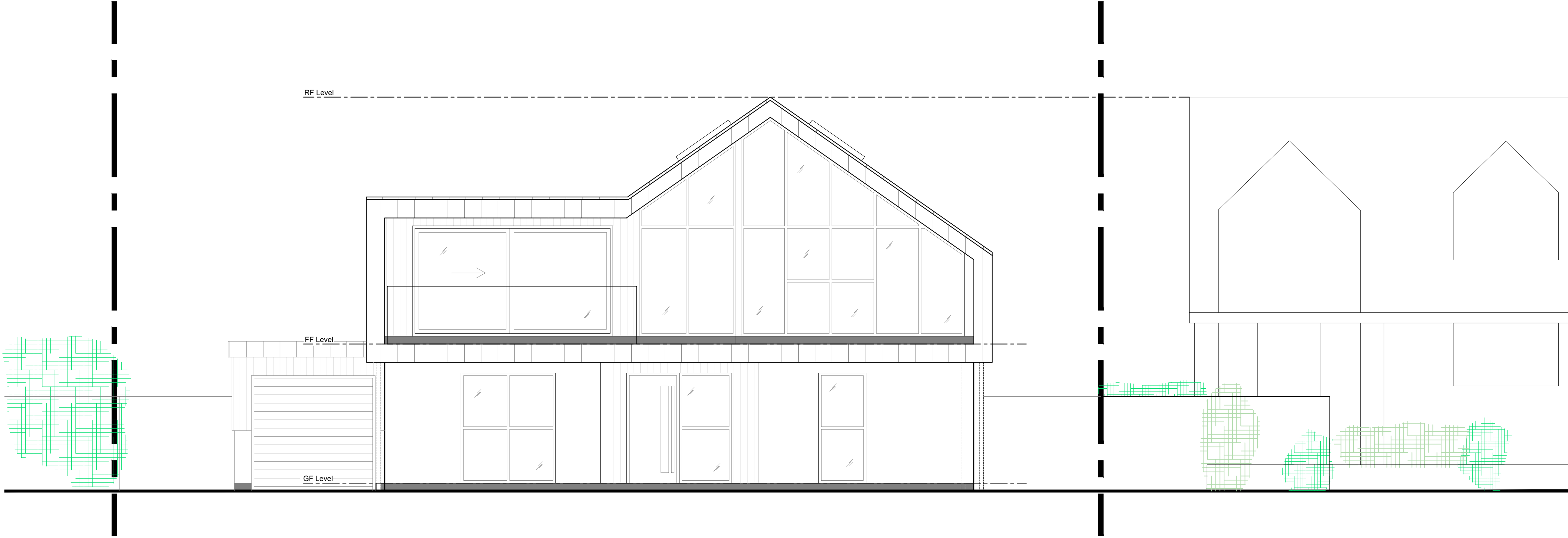
FRONT ELEVATION
