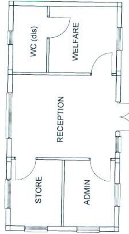
WELFARE PLAN 1:100
