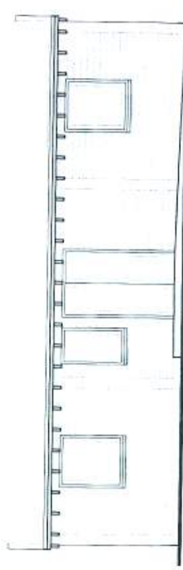
WELFARE SOUTH ELEVATION 1:100
