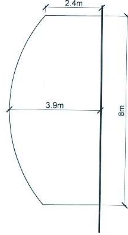
TYPICAL END ELEVATION 1:100
