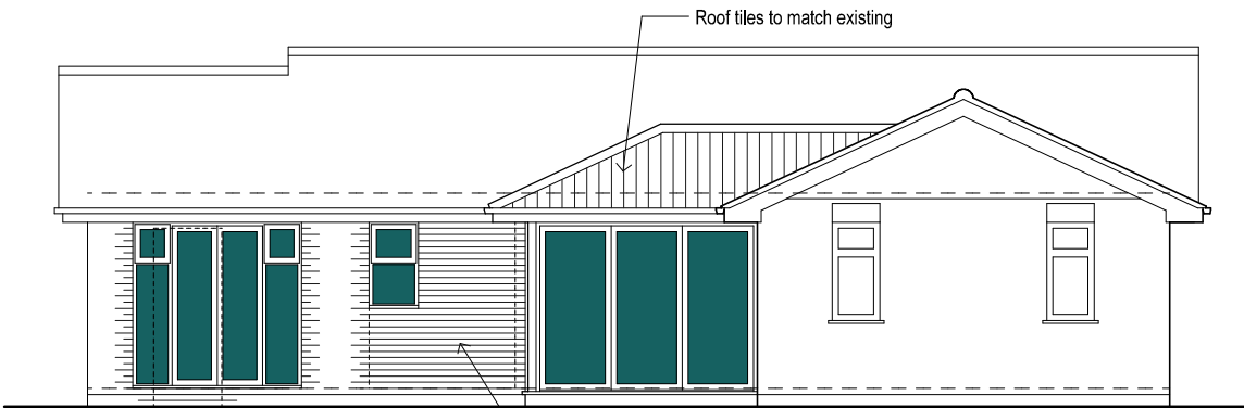
South Elevation - Proposed
