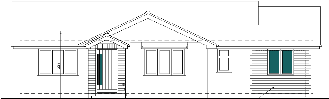
North Elevation - Proposed
