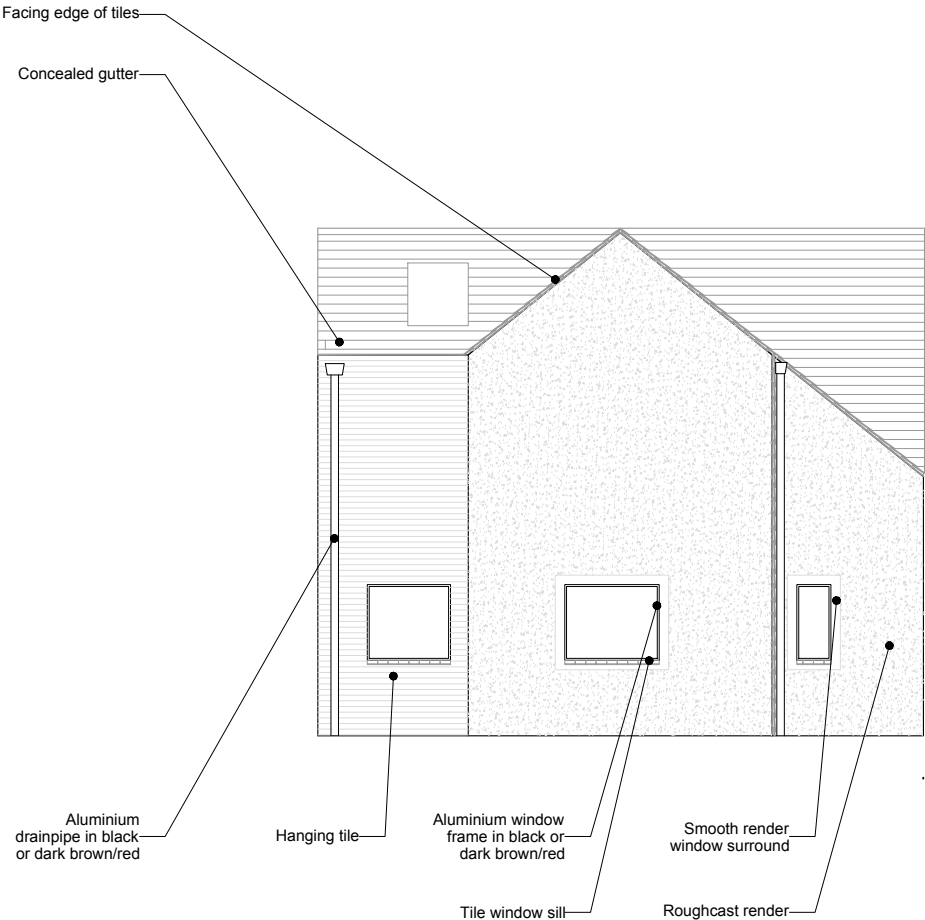
North Elevation
