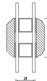
56mm BONDED BARS
