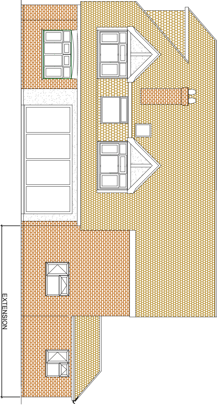
SOUTH ELEVATION
