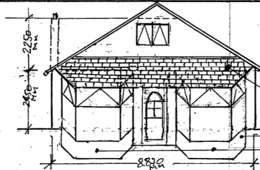
PROPOSED FRONT ELEVATION SCALE 1:100
