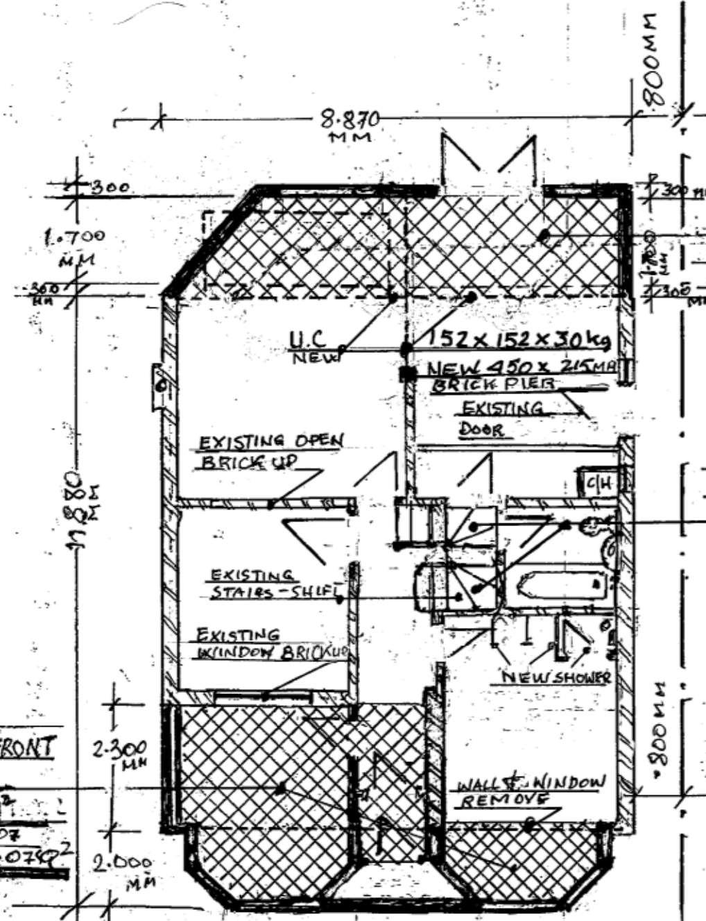
PROPOSED GROUND FLOOR SCALE 1:100 PLAN
