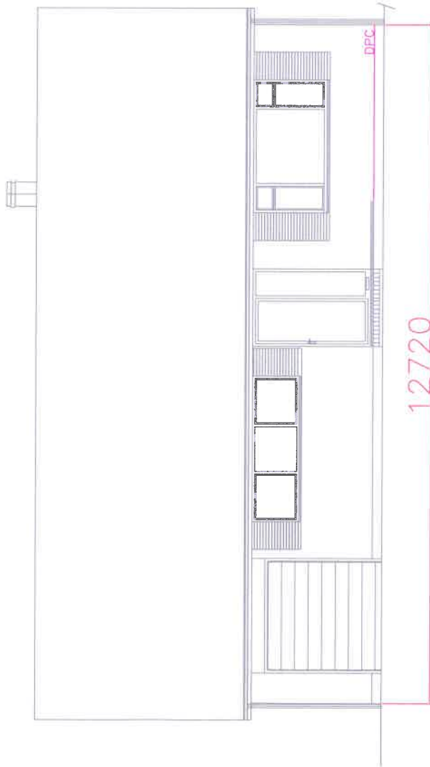
EXISTING NORTH ELEVATION
