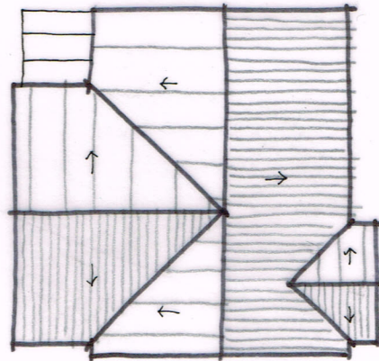
ROOF PLAN 1:200
