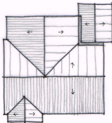
ROOF PLAN 1:200
