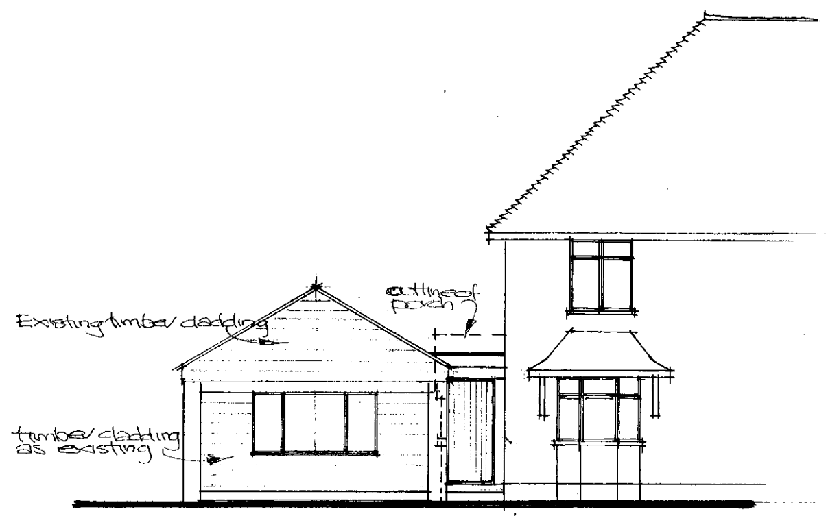
Proposed North Elevation - scale: 1/100
