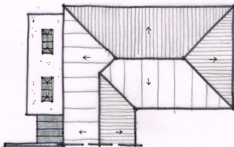
ROOF PLAN 1:200
