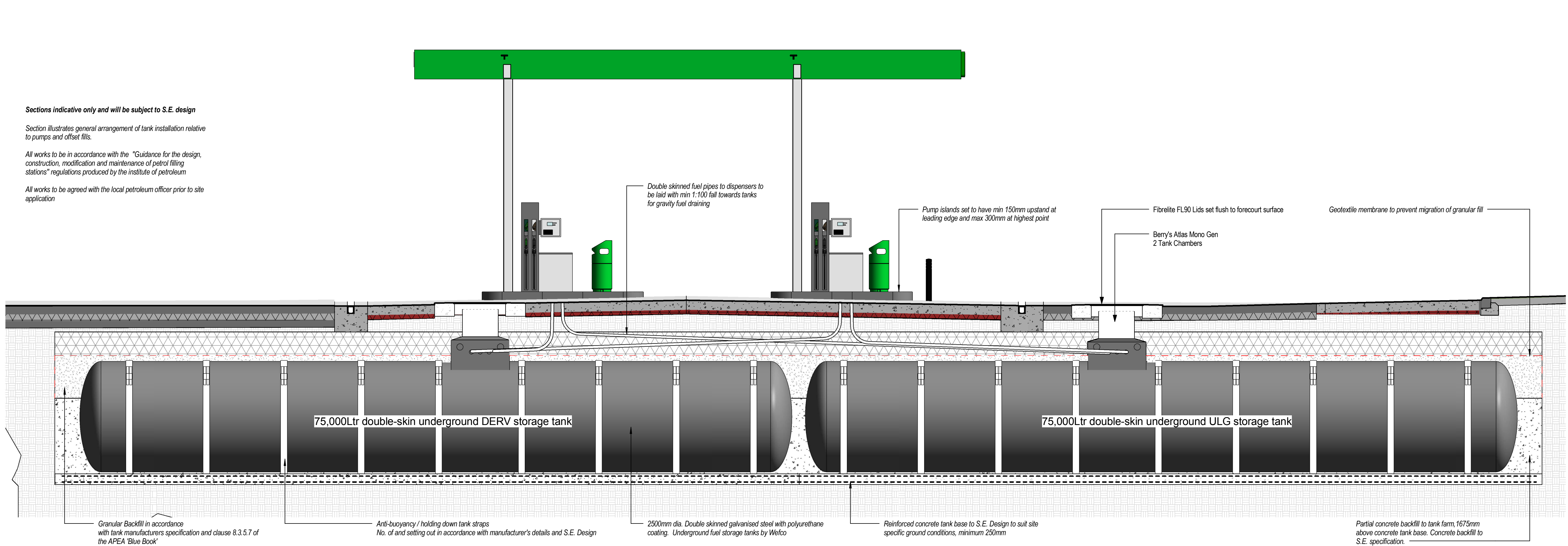
Forecourt Cross Section Copy 1 1 : 50
