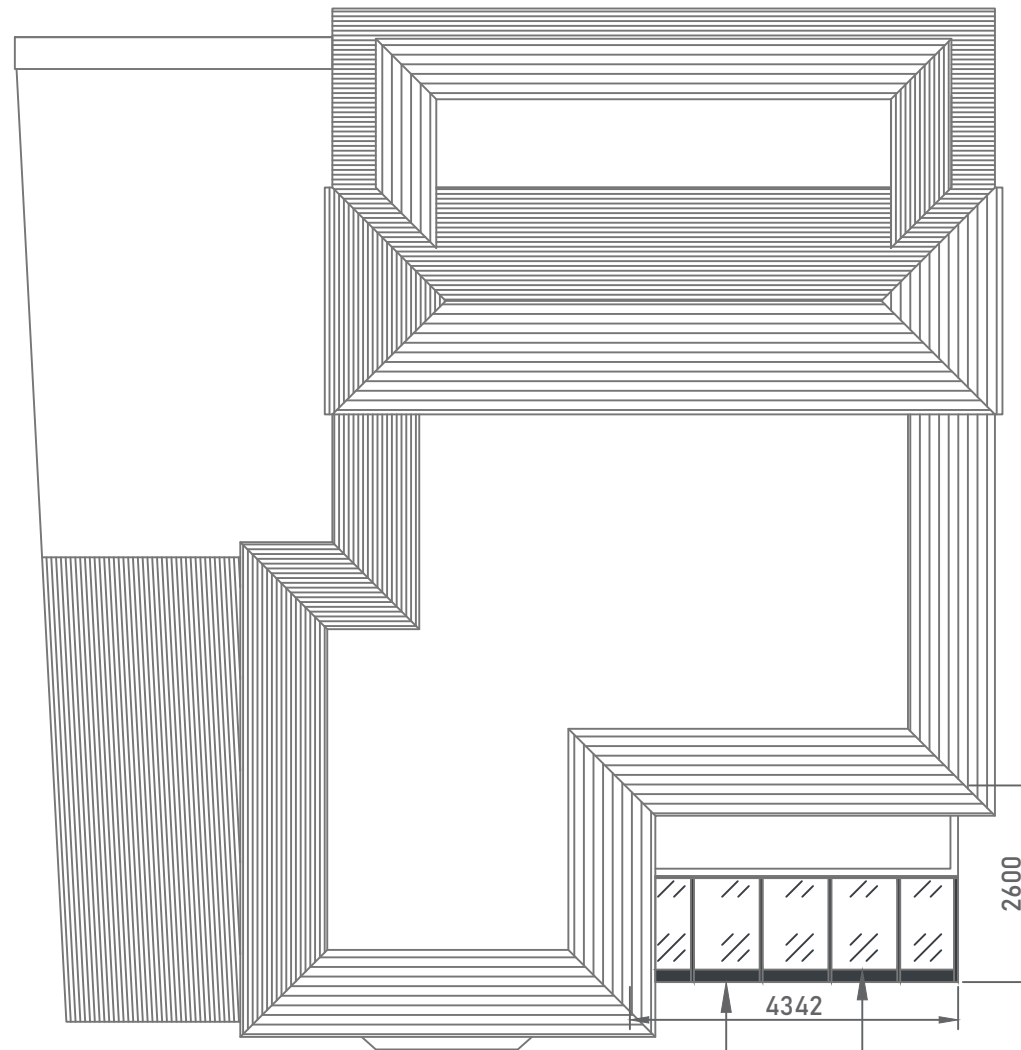
ROOF PLAN
