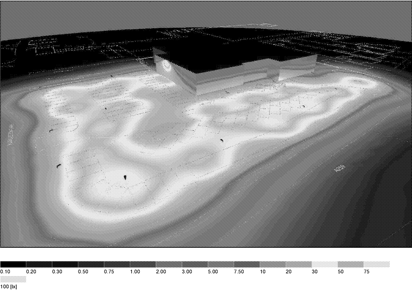
Site 1 (6), Illuminance values in [lx]
