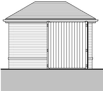
Rear Elevation
