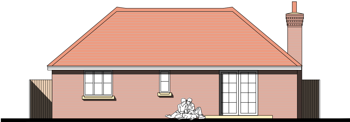
West Elevation
