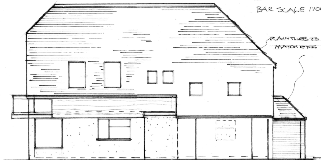
EAST ELEVATION 1:100
