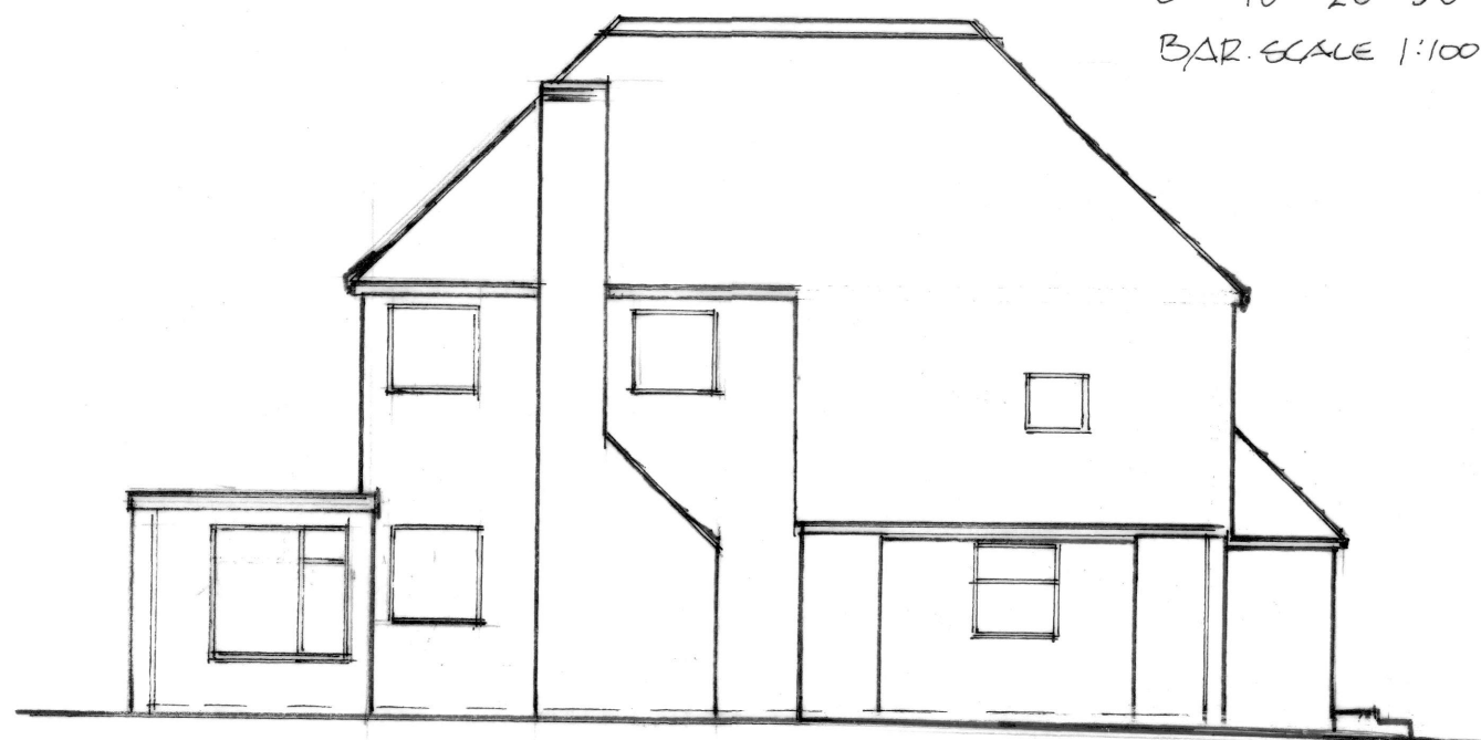
EAST ELEVATION 1:100
