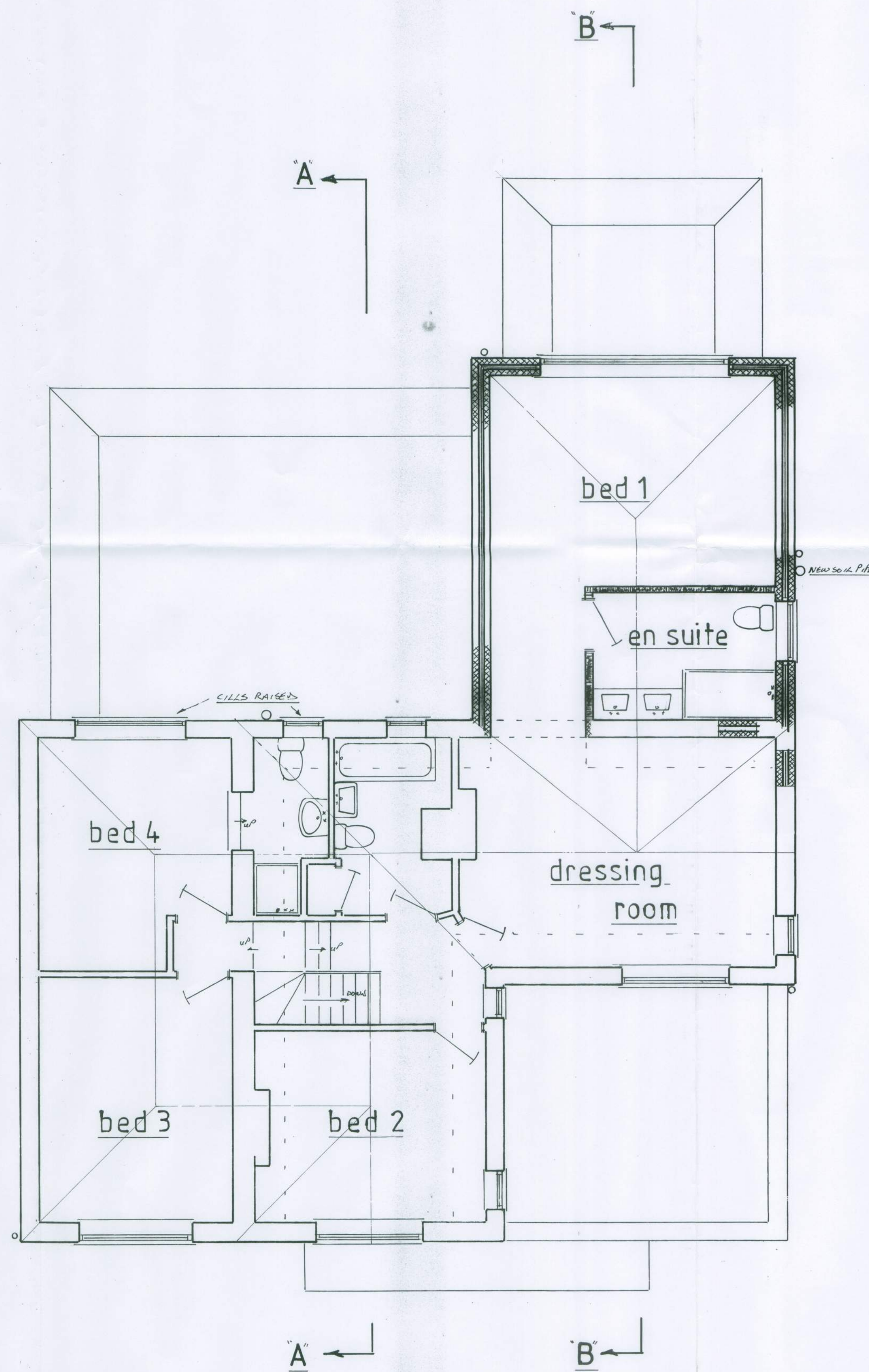
First Floor
