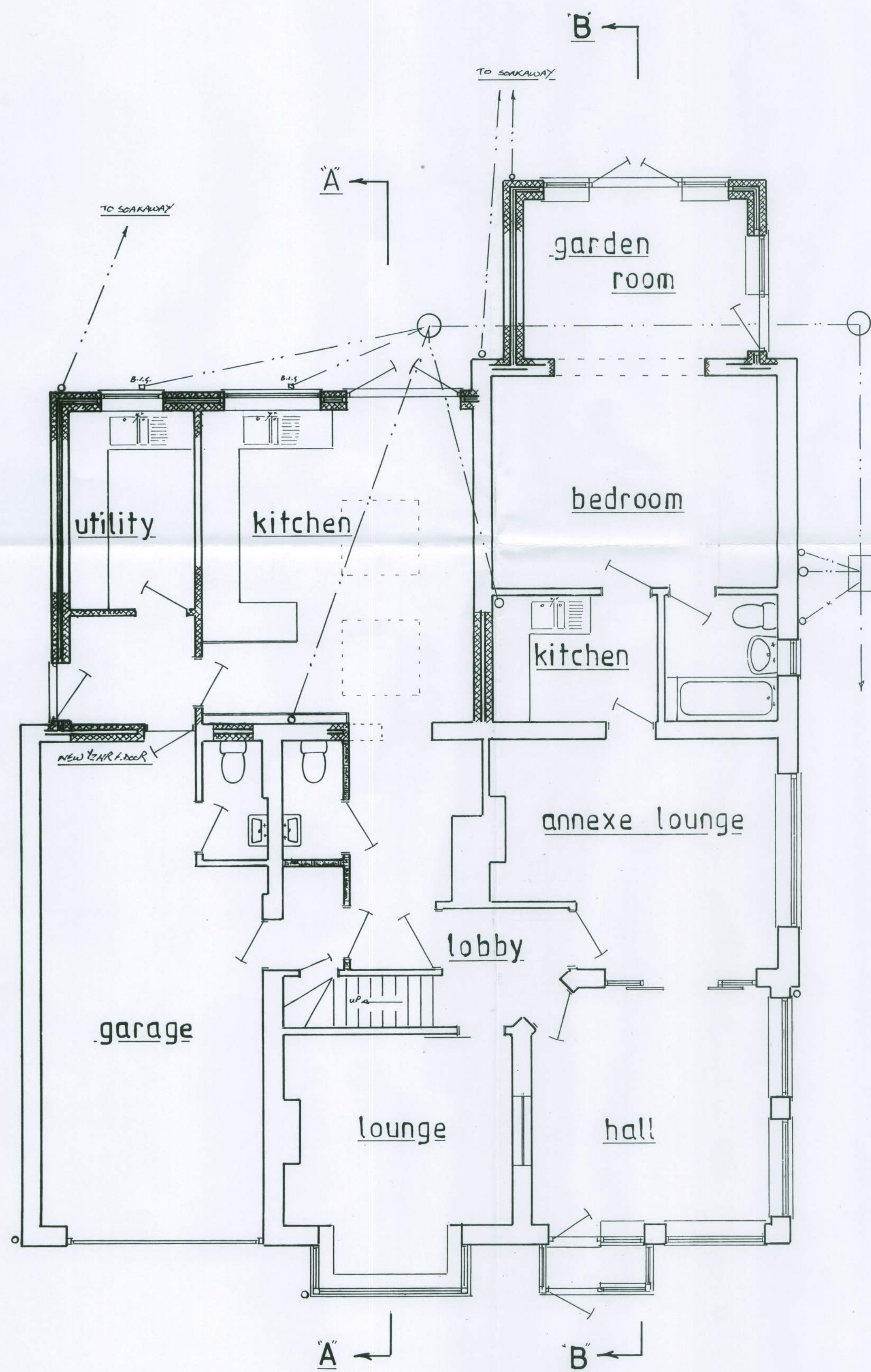
Ground Floor
