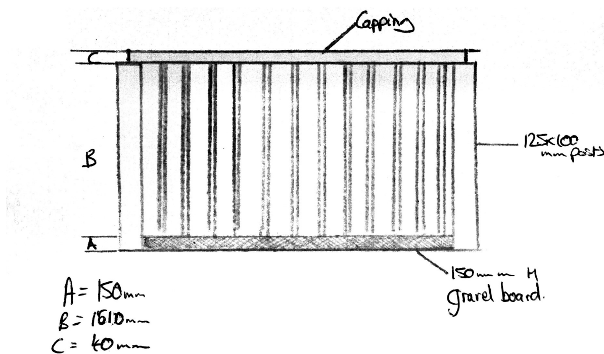
Sketch illustrating height and composition of acoustic fence
