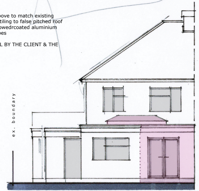
REAR (n)
