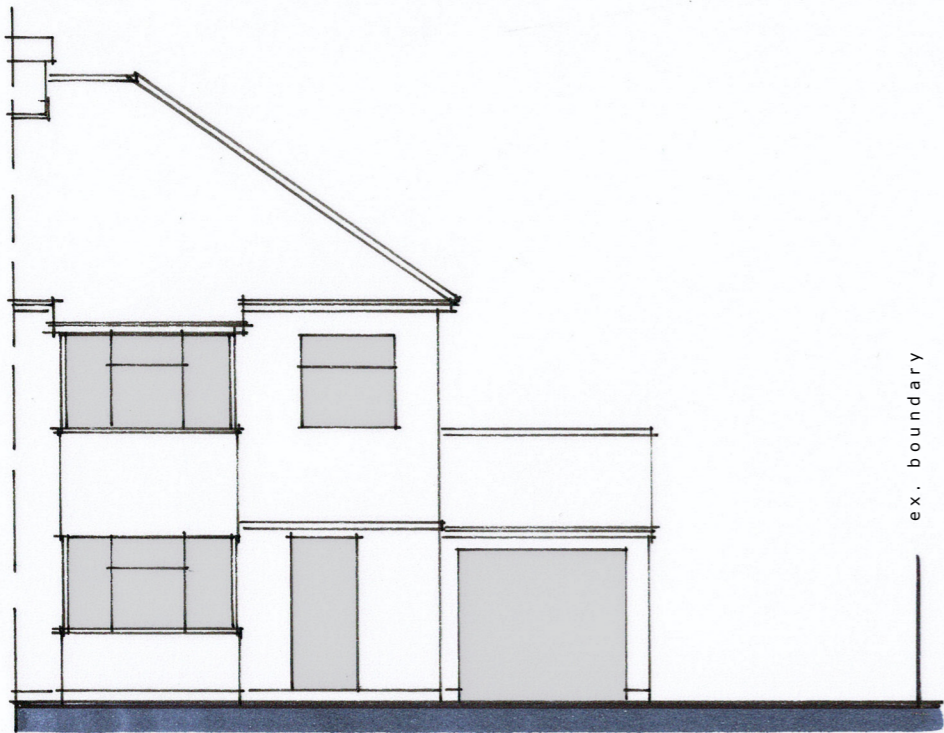
FRONT (s)
