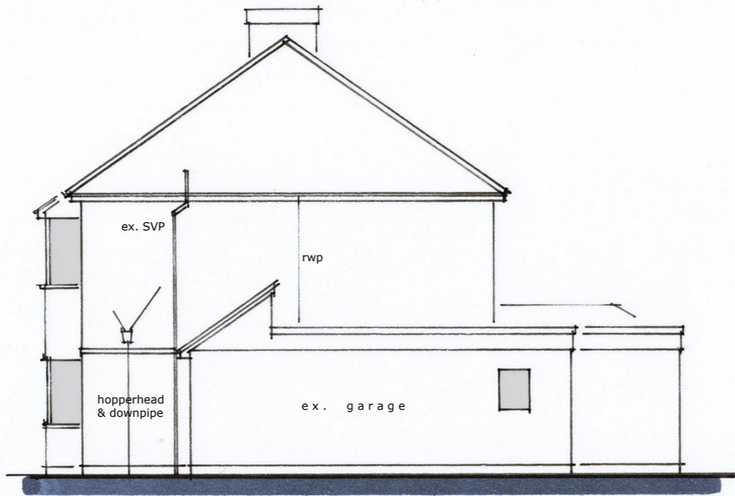
SIDE (e) ELEVATION 1:100 @ A3
