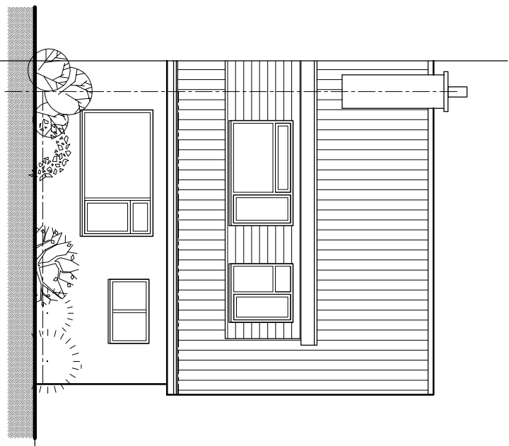
South Elevation
