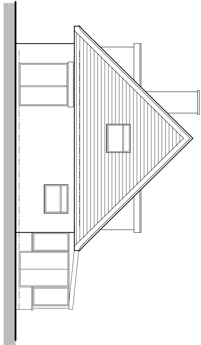
East Elevation
