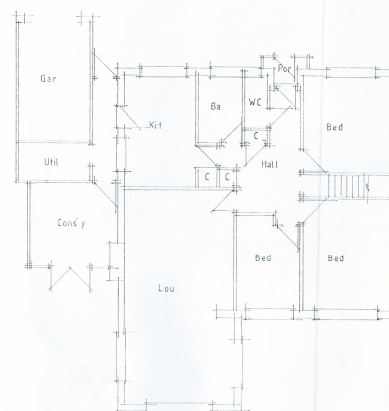
Existing plan 1:100
