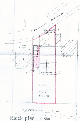
Block plan 1:500
