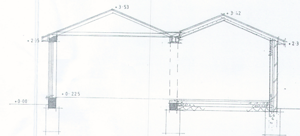
Section AA 1:50
