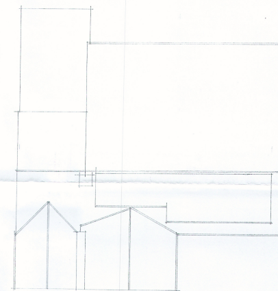
Roof proposed 1:100
