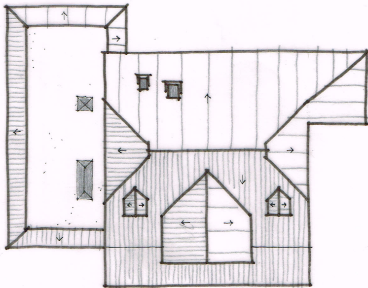
ROOF PLAN 1:200
