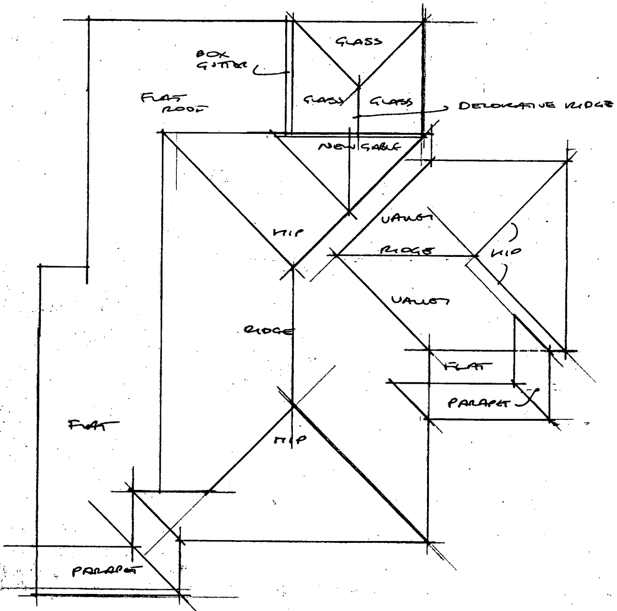
Roof plan 1:100 60 Cissbury Road : Ferring
