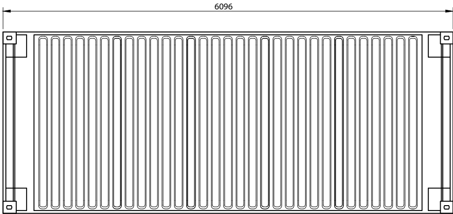
Roof Plan
