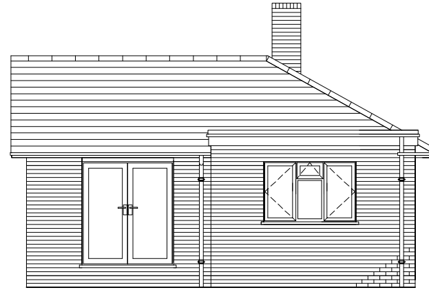
Rear Elevation (North East Facing) (Scale 1:100)
