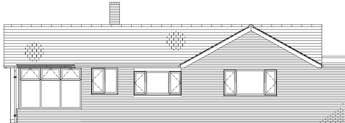
Side Elevation (South East Facing) (Scale 1:100)
