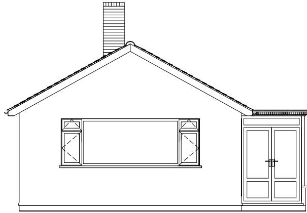
Front Elevation (South West Facing) (Scale 1:100)
