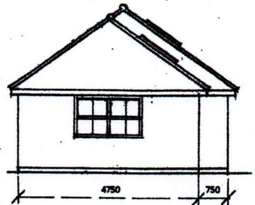
NORTH (SIDE)
